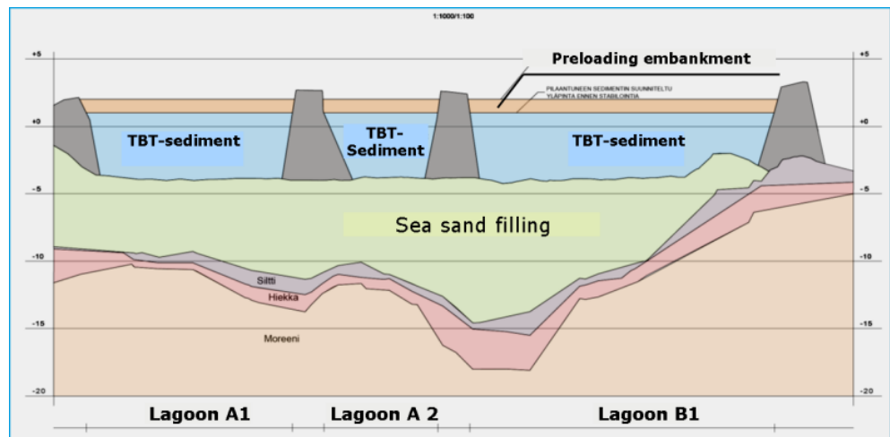
The principle of utilizing sediments in Vuosaari.
